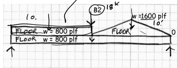
Load diagram
