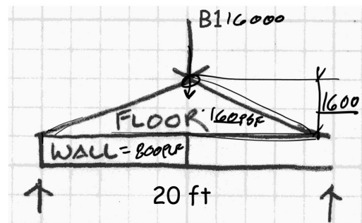
Load diagram
