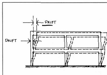
Story-to-story drift
