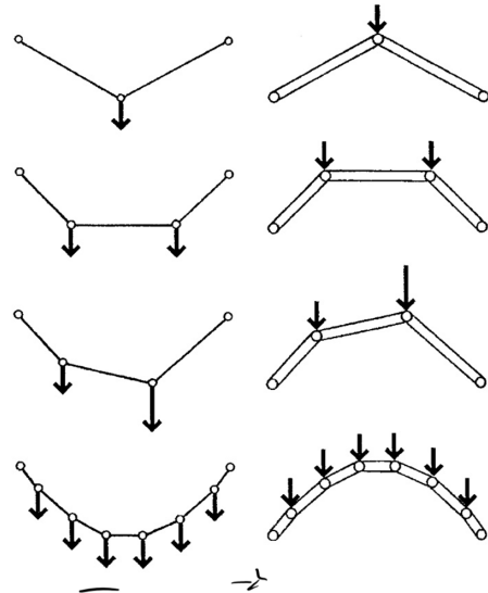
Funicular suspension cables and corresponding arches.
