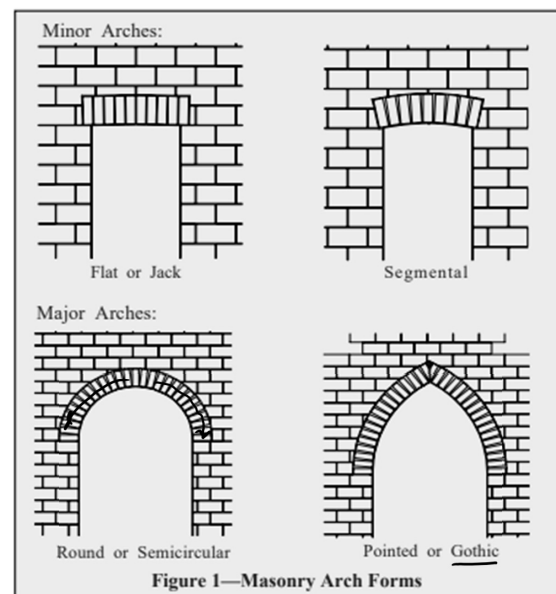
Figure 1—Masonry Arch Forms
